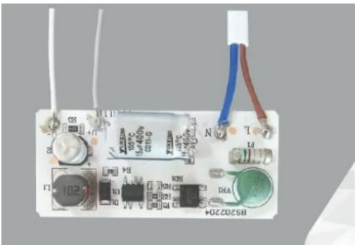
38W driver-DOP without leading wires/connectors
