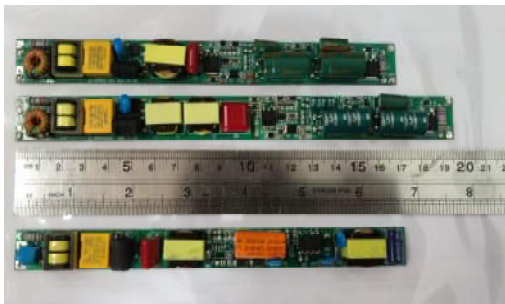
25W driver-A
